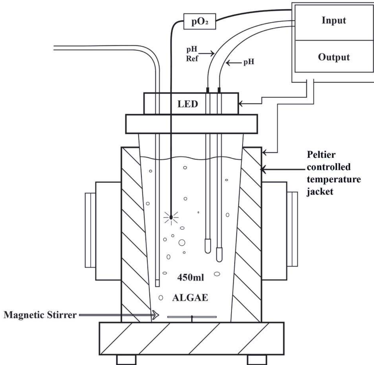
Figure 1. Phenometrics ePBR schematic diagram. Light intensity is controlled using a white light LED array and culture temperature is controlled with a Peltier controlled temperature jacket. The PBR is comprised of a magnetically-stirred chamber, filled with a 10% v/v N. oculata stock culture inoculum in f/2 medium. Aeration with ambient air is supplied through a gas dispersion tube. Dissolved oxygen (pO 2 ) is measured optically (PyroScience) and pH is measured electrochemically (Phenometrics). doi:10.1371/journal.pone.0086047.g001
